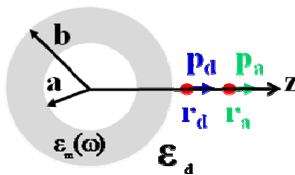
Fig. 1(b): Schematic picture showing a pair of two level molecular system (labeled acceptor-a, and donor-d for definiteness) in the proximity of NSH monomer of inner and outer radii, a and b , respectively. Other parameters are the same as in Fig. 1(a).
